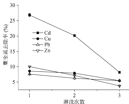
图 4 连续提取对 EDTA 去除土壤重金属效率的影响 Fig. 4 Extraction efficiency of 3 cycles of successive 1 h extractions with EDTA (liquid: solid = 2.5)
