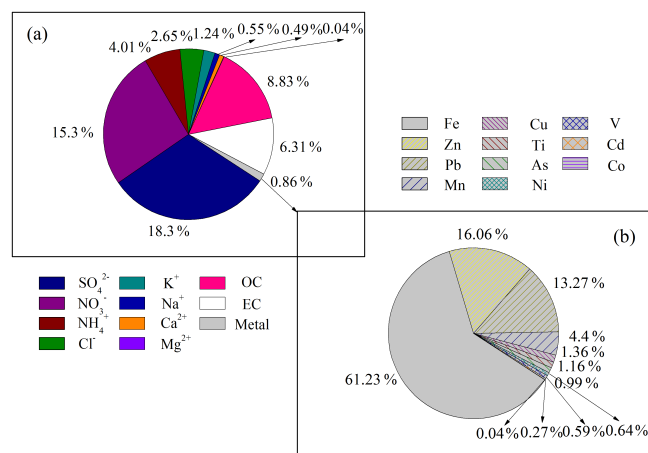
Figure 3. Pie charts showing the relative contribution of species for PM 2.5 in Qimu Island. Note the sum of percentage of identified species in PM 2.5 in (a) is 58.58 %, while that in (b) is 100 % because the percentage is the ratio of every metal element to the total identified metal elements.
