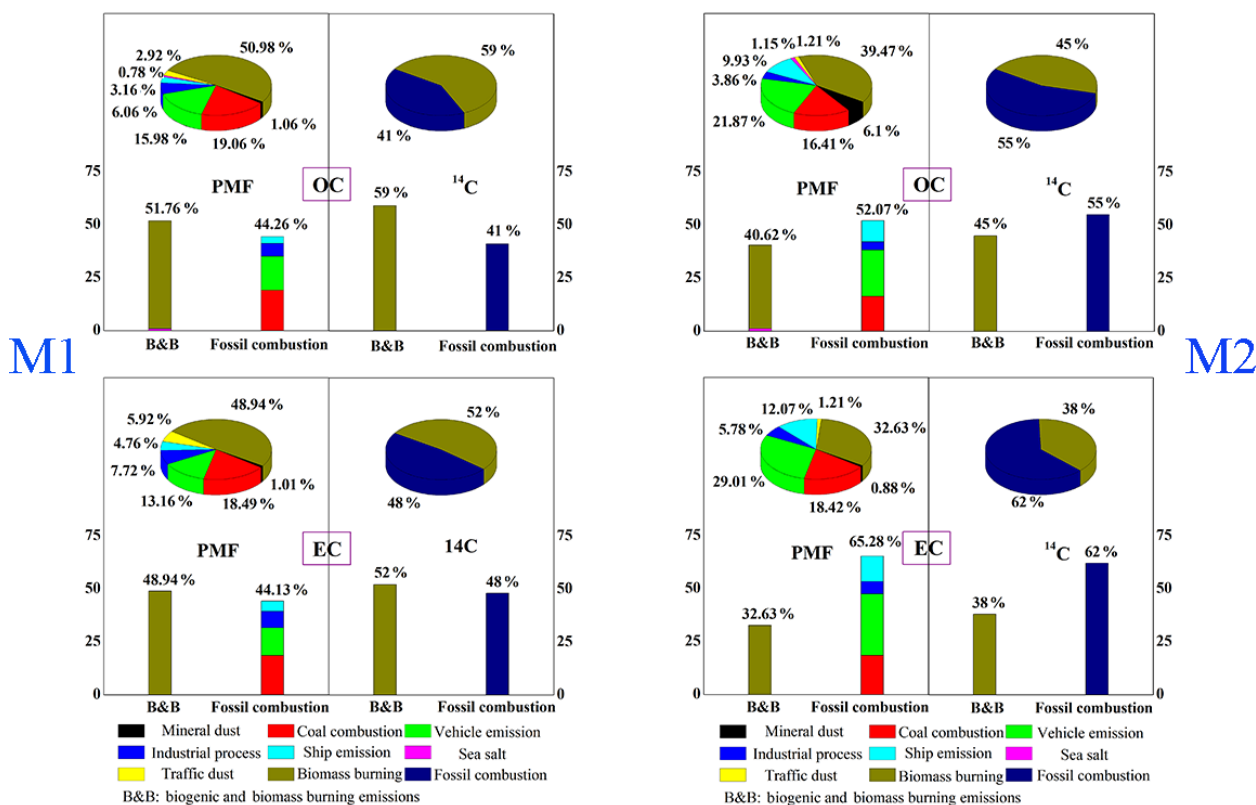
Figure 5. Comparison of source apportionment of OC and EC in the two specified samples (M1 and M2) from PMF and 14 C measurement. B&B refers to the source of biogenic and biomass burning. Note: B&B and fossil emissions from the PMF result do not add up to 100 in the bars because hybrid sources from B&B and fossil fuel combustion were not considered in the comparison (mineral dust and vehicle dust).
